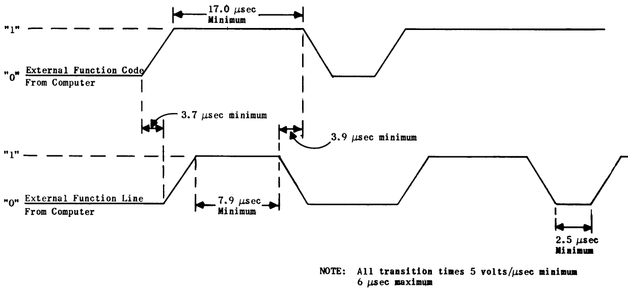
Figure 12. Timing for External Functions with Force - Slow Interface
