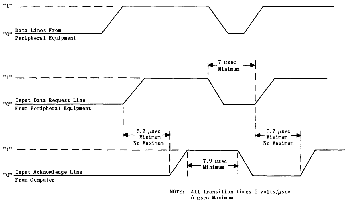
Figure 9. Timing of Input Data Signals - Slow Interface
