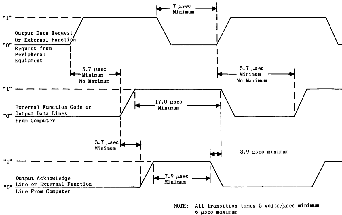
Figure 11. Timing for Normal Output Signals - Slow Interface
